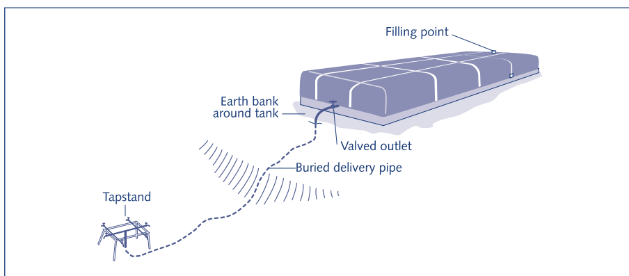
Fig. 24.2. Typical set-up of a distribution point in a tankering operation Source: Davis, J. and Lambert, R., 2002
