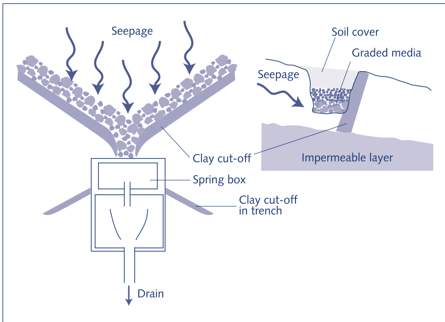
Fig. 24.10. Seepage spring protection Source: Davis, J. and Lambert, R. 2002
